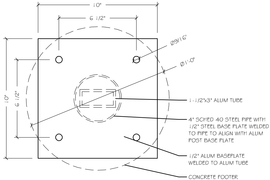
2 DETAIL-BASE PLATE 3" = 1'-0"
