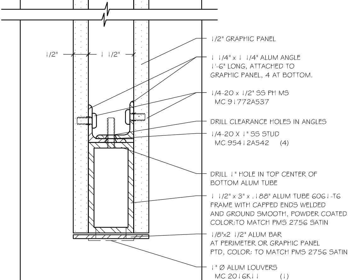
A SECTION HALF
