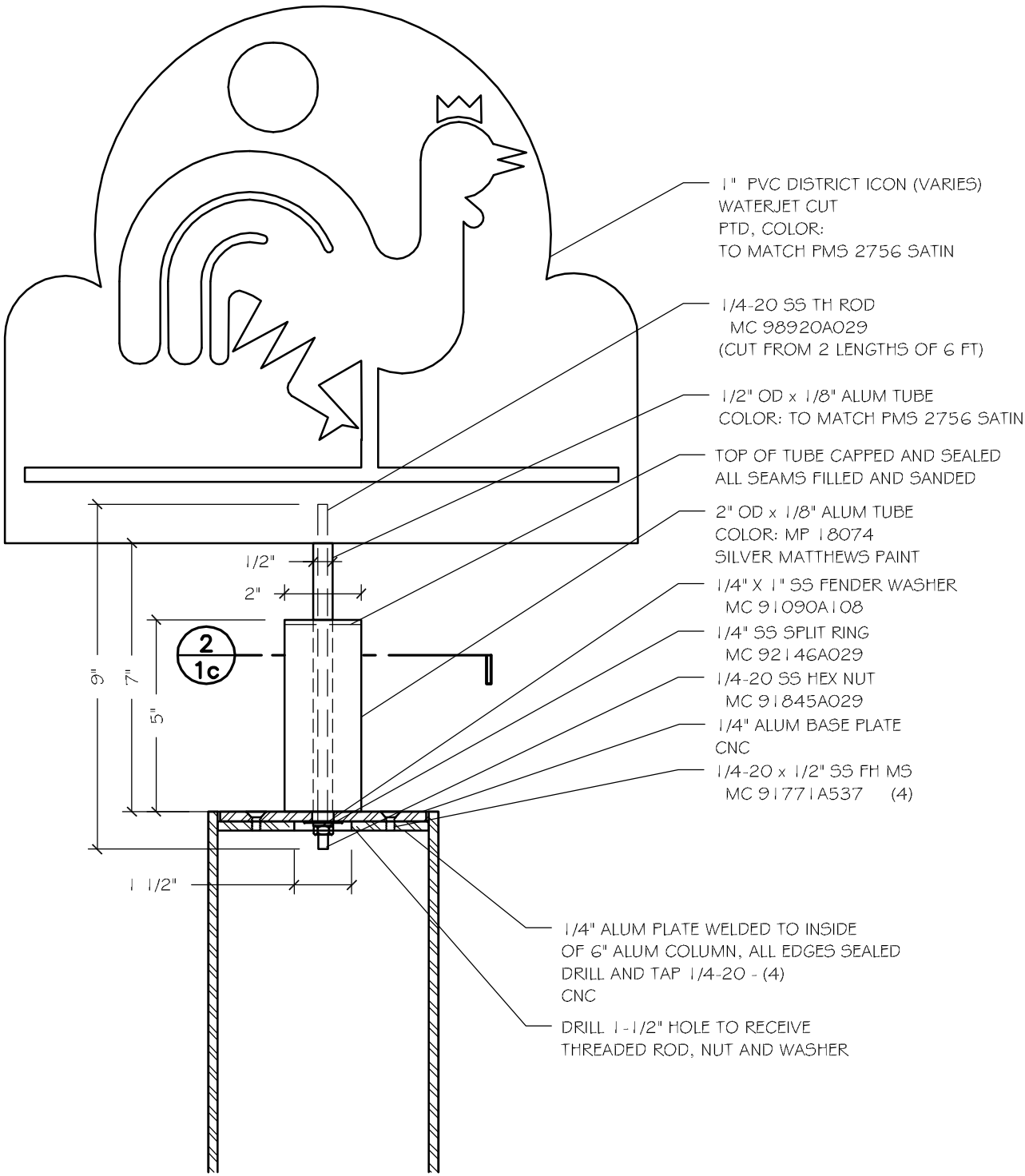
1 SECTION-ELEVATION 3" = 1'-0"
