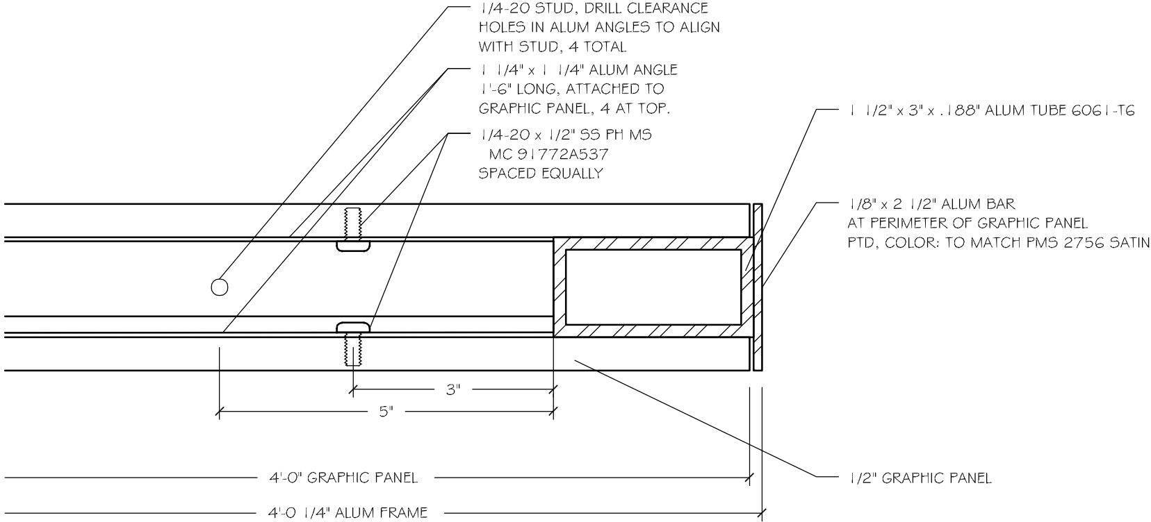
B SECTION HALF
