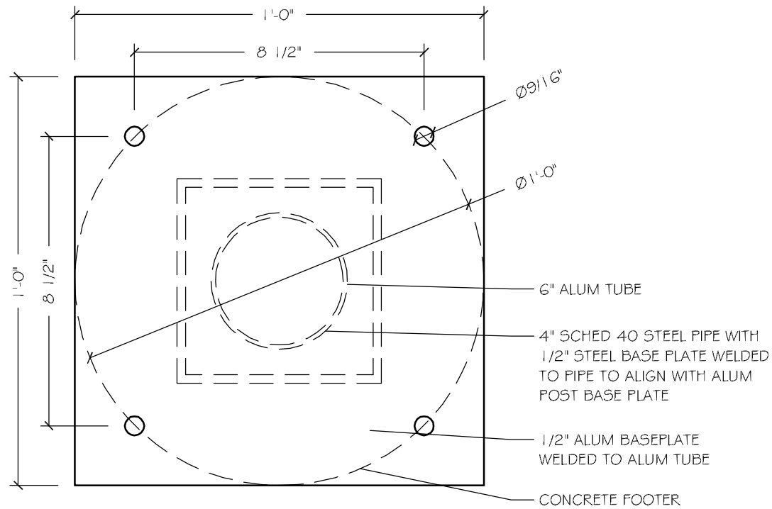
1 DETAIL-BASE PLATE 3" = 1'-0"
