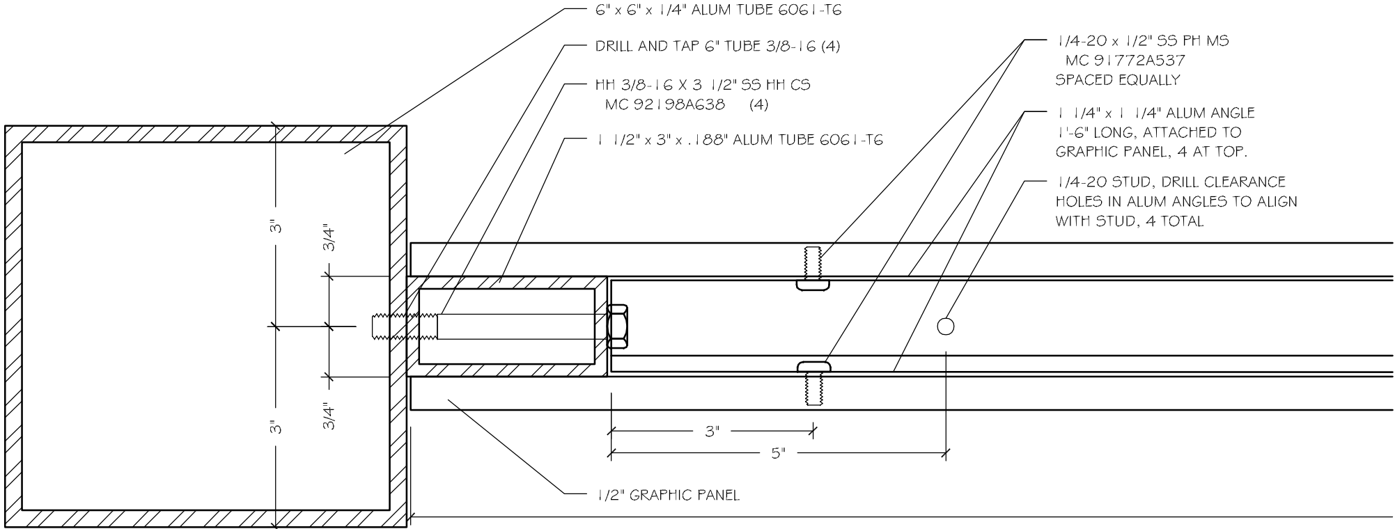
A SECTION HALF
